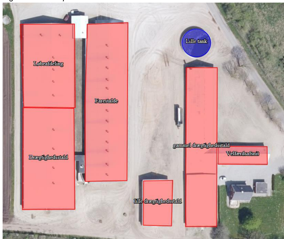
Figur 1 Situationsplan
